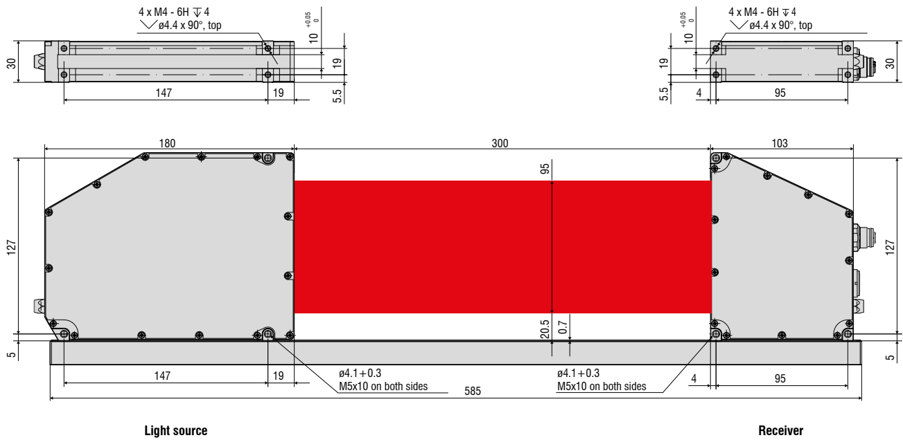
Light source
